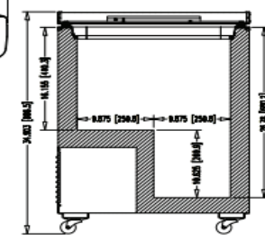
SECTION VIEW
