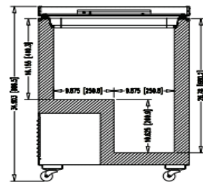
SECTION VIEW
